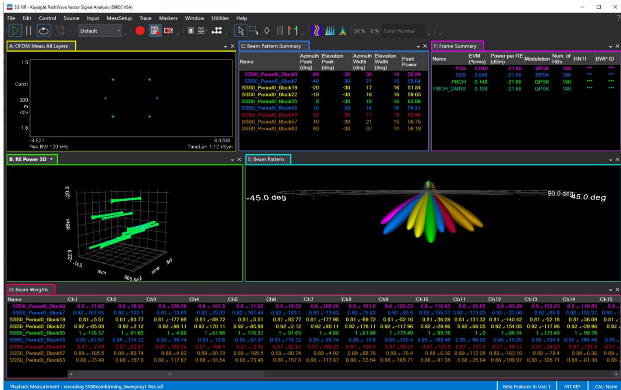
Figure 9. Example of downlink beamforming with magnitude and phase weightings and corresponding beam patterns.
