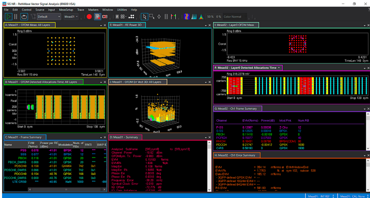
Figure 10. VSA's DSS analysis capability shows demodulation of 5G NR and LTE carriers and side-by-side presentation of measurement results.
