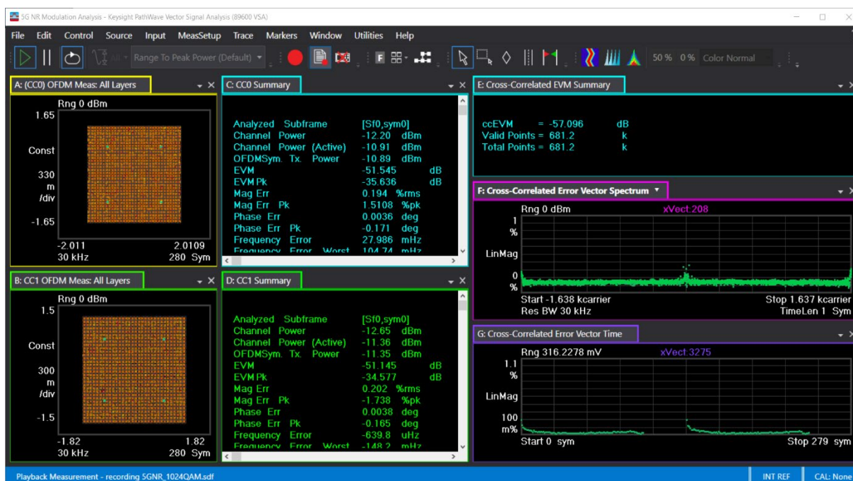
Figure 11: Cross-correlated EVM (Trace E) compared with EVM of individual receiver (Trace C and D). In this loop back example of a signal generator and two receivers, ccEVM results in a 5.5 dB EVM improvement of a 100 MHz, 1024QAM Test Model NR signal.
