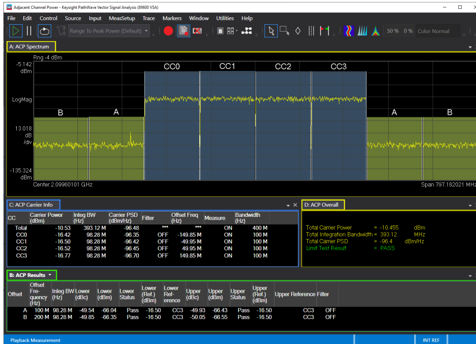
Figure 12. 5G NR multi-carrier ACP measurement with four contiguous component carriers
