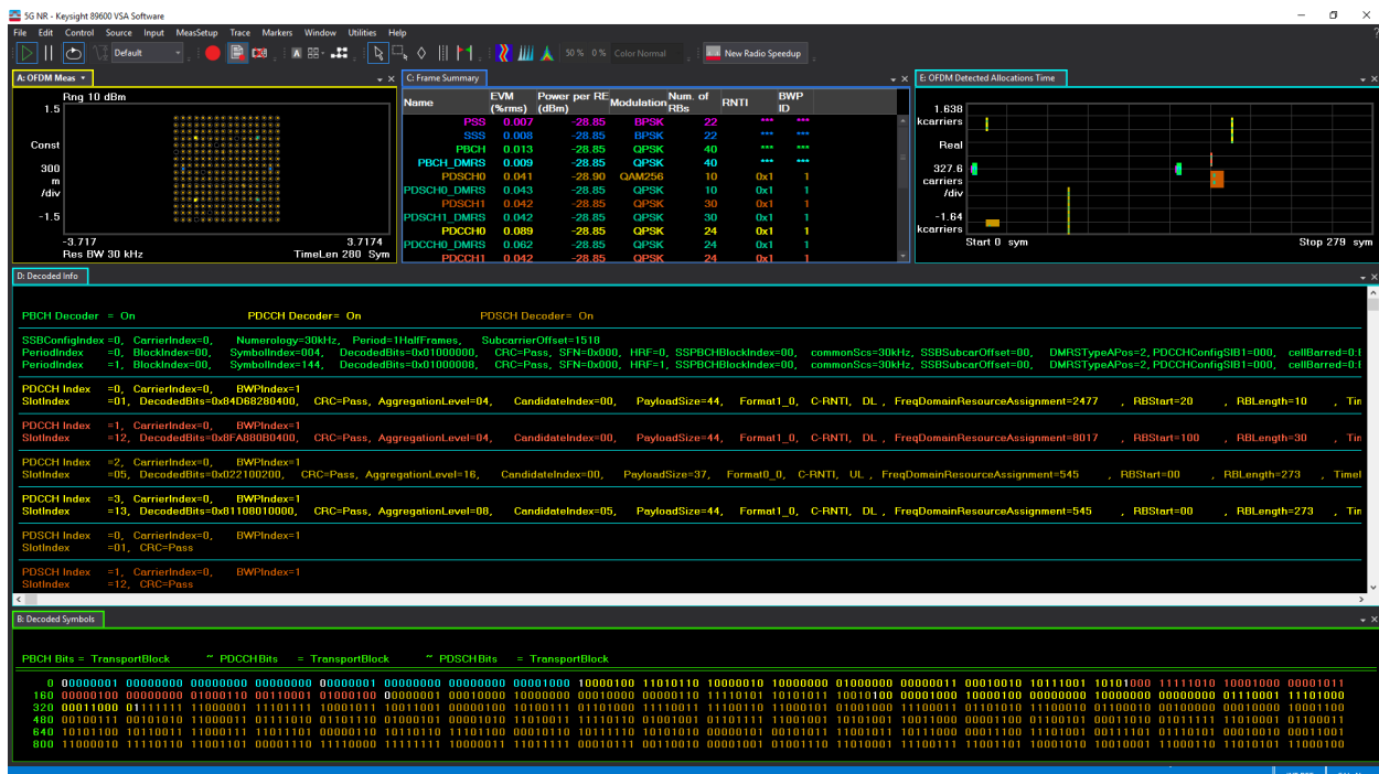
Figure 4. Example of a downlink decoded information and decoded symbols for PBCH, PDCCH and PDSCH.
