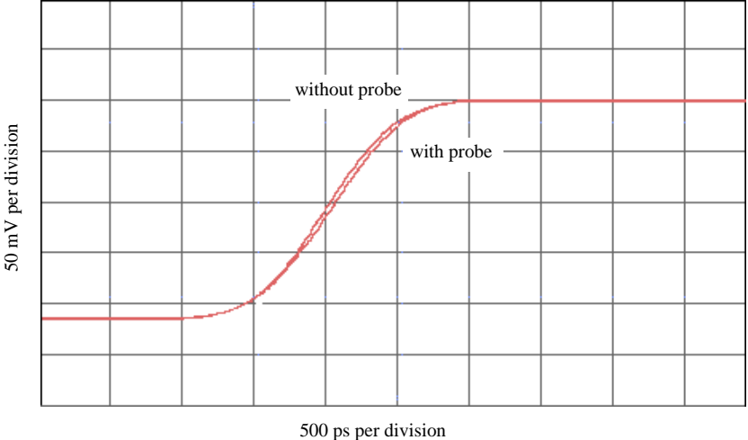
Figure 52 TDT measurement at receiver with and without probe load for 1 ns rise time
