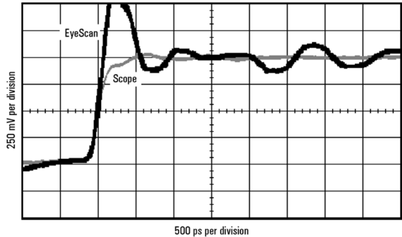
Figure 74 Logic analyzer's response to a 500 ps rise time
