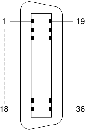
Connector pin No. assignment
