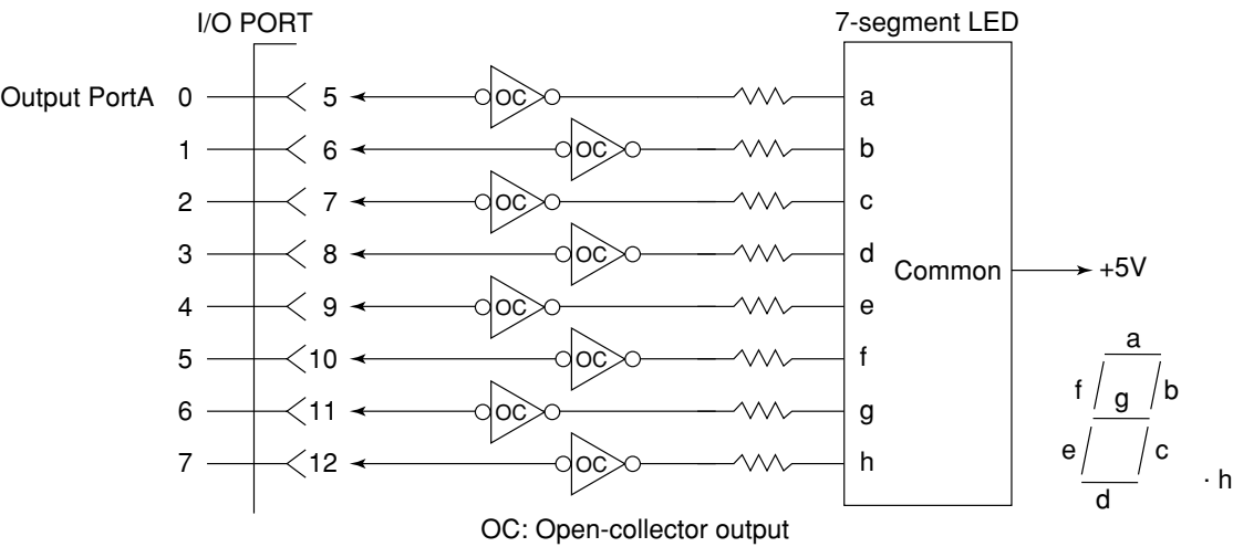
Curcuit example 2:
