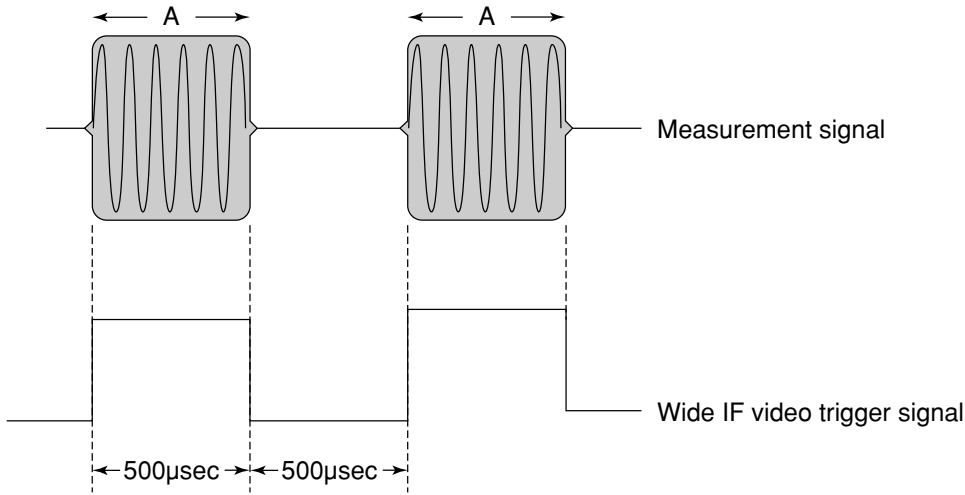
Fig. 6-1 Burst Waveform
