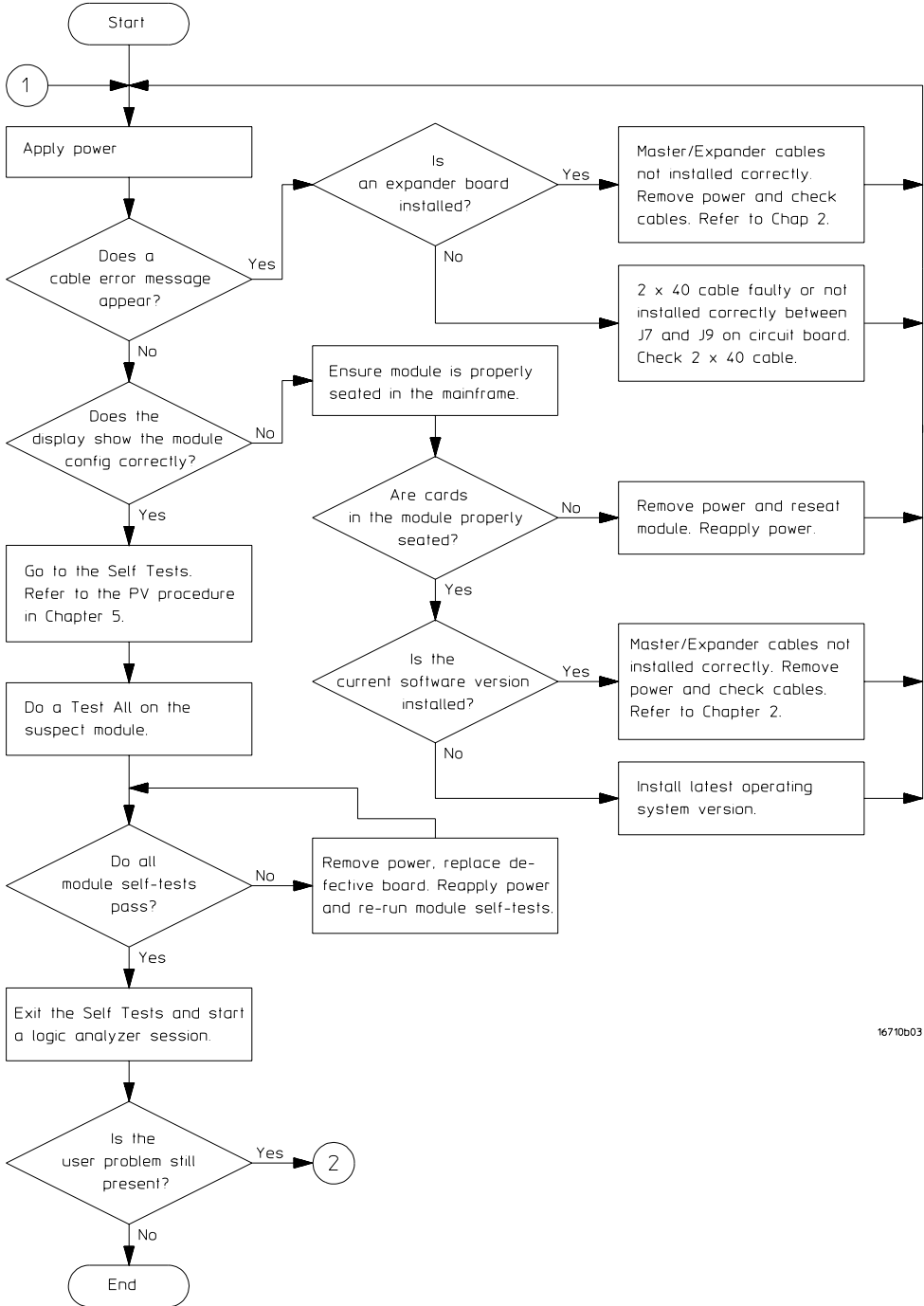
Troubleshooting Flowchart 1
