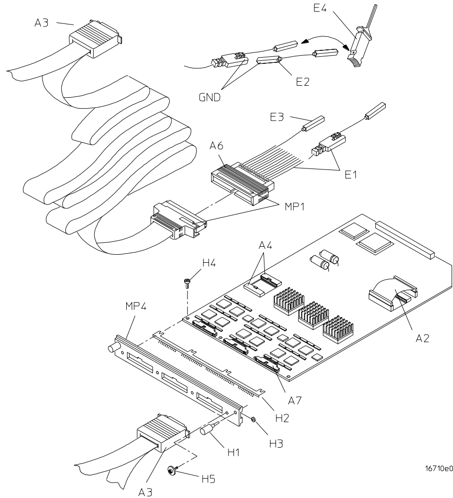
Exploded view of the 16710A/11A/12A logic analyzer
